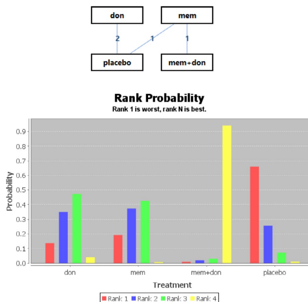
FIGURE 4 Network meta-analysis on Alzheimer's disease treatment. Assessment of the change in the clinical global impression. Don, donepezil; mem, memantine; mem + don, combination of donepezil and memantine; CGI, clinical global impression; MD, standardized mean difference; CrI, credible interval
